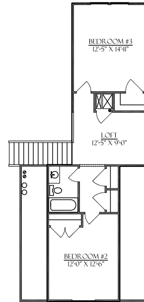
UPPER FLOOR
