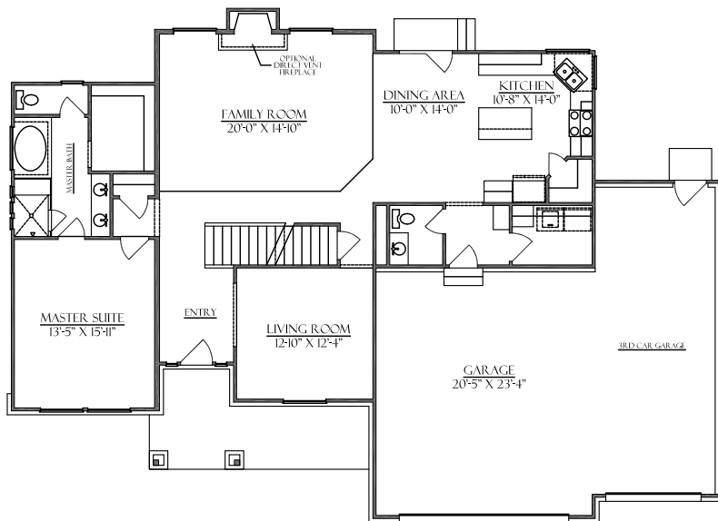
MAIN FLOOR
