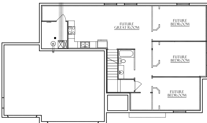
BASEMENT FLOOR
