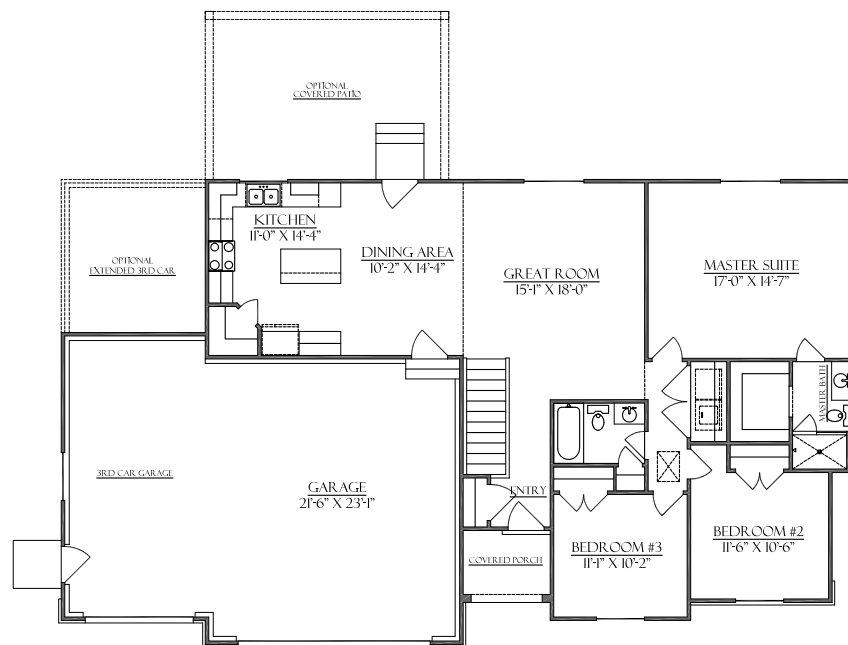
MAIN FLOOR
